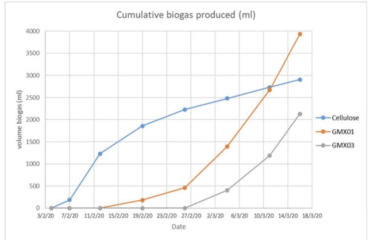
Figure 2: Graph to illustrate gas yield over time for the cellulose, GMX01 and GMX03
